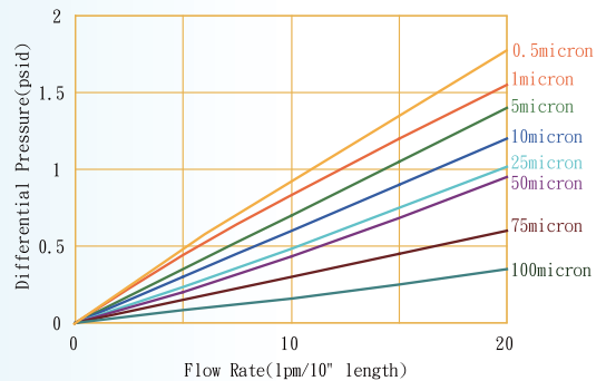
Flow vs. Differential Pressure
