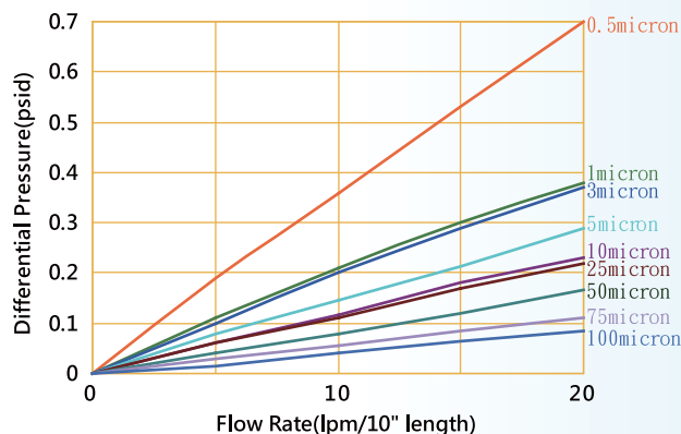
Flow vs. Differential Pressure
